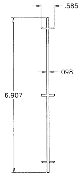
4 MULLION
