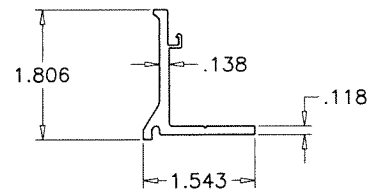
2 GLASS STOP
