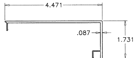
3A FRAME COVER (INSUL. LAM. GLASS)
