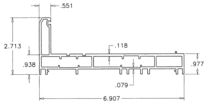
1 FRAME HEAD/SILL/JAMB
