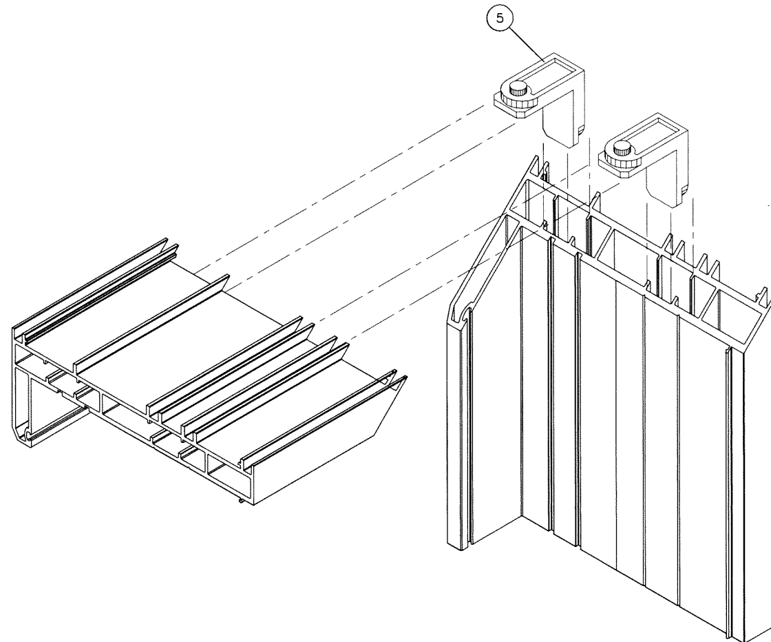
FRAME CORNER
